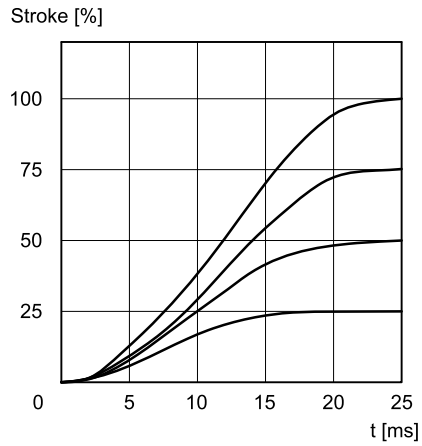
RESPONSE TIME
