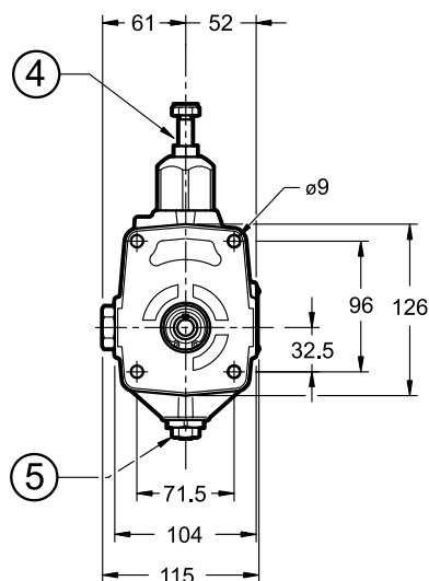
RV1D-016PC-R97B
