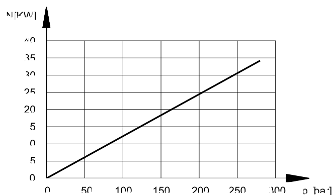
ABSORBED POWER
