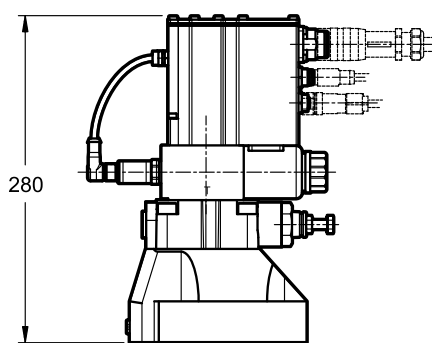
PRE32JH
