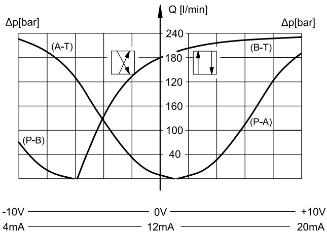
SPOOL X1A220
