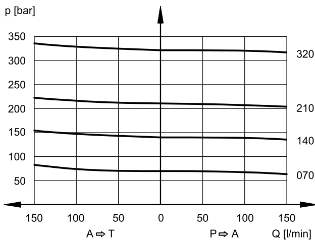
CONTROLLED PRESSURE
