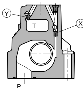
DZC8
