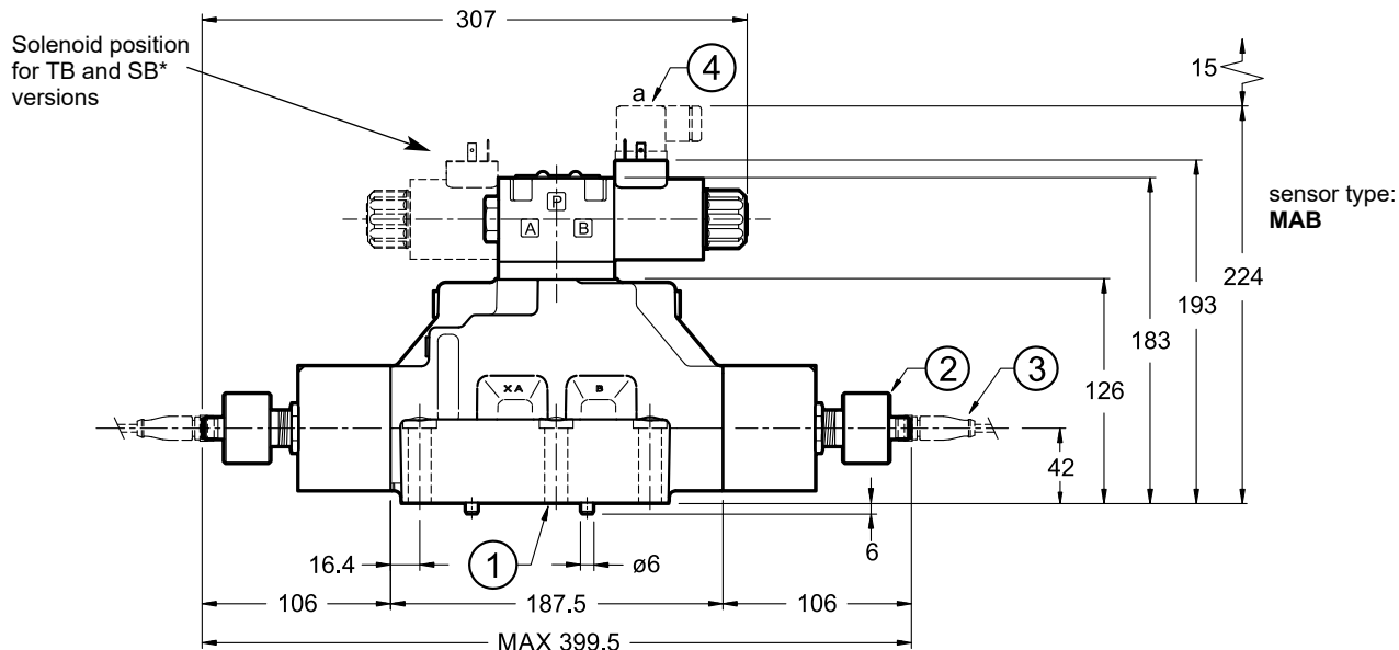
DSP8M-TA, TA100, SA1
