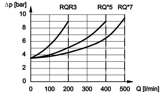
MINIMUM CONTROLLED PRESSURE
