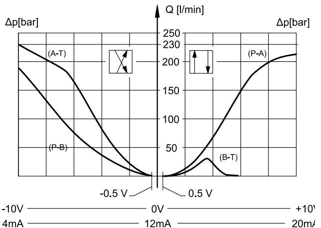
SPOOL R1C220 / R1A220
