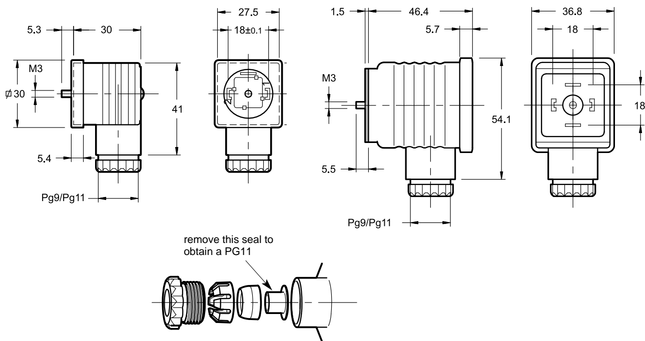
type A, B1, B2, D
