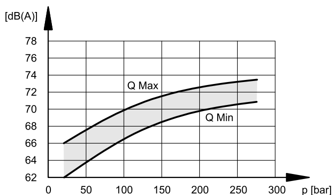
NOISE LEVEL
