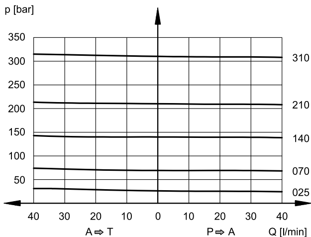
SET PRESSURE
