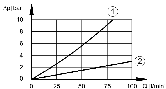
PRESSURE DROP \Delta p = f(Q)
