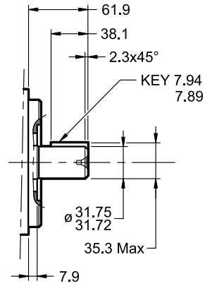
cylindrical keyed - no SAE (identification code: 2)
