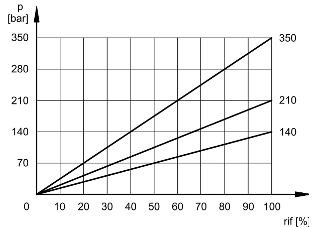
PRESSURE CONTROL p = f(l)
