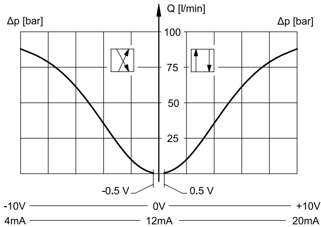
SPOOL C100 / A100
