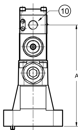
PRE25K*-/20*-*K9S*
