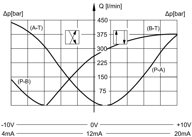
SPOOL X1A430
