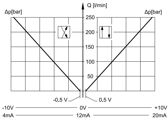
SPOOL X1A430
